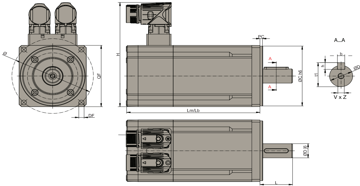
Dimensions [mm]
